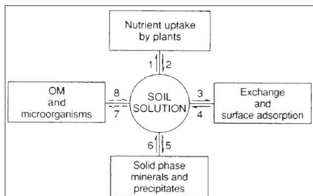
Fig 1: 1 = absorption, 2 = exudation, 3 = adsorption, 4 = desorption, 5 = precipitation, 6 = dissolution, 7 = immobilization, 8 = mineralization
