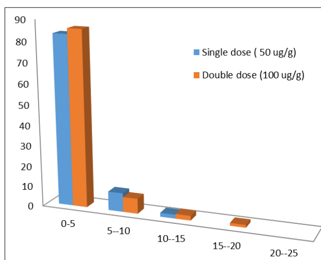
Fig 1: leaching potential of ready-mix formulation of thiamethoxam in soil and in leachates
