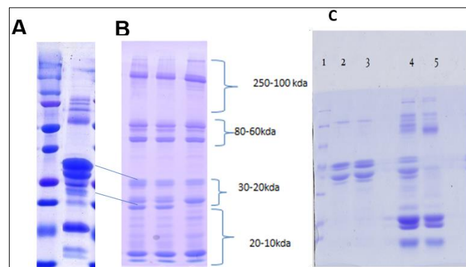
Fig A, B, C: (A) band pattern of whole milk protein after the removal of fat Lane 1: Marker Lane 2: Defatted whole milk protein (B) Band pattern of milk protein after casein removal by ultracentrifugation Lane 1, 2 & 3: proteins after casein removal (C) Comparison of casein removal methods Lane1= Protein marker Lane2, 3= removal of casein by low pH Lane 4, 5=removal of casein by ultracentrifugation
