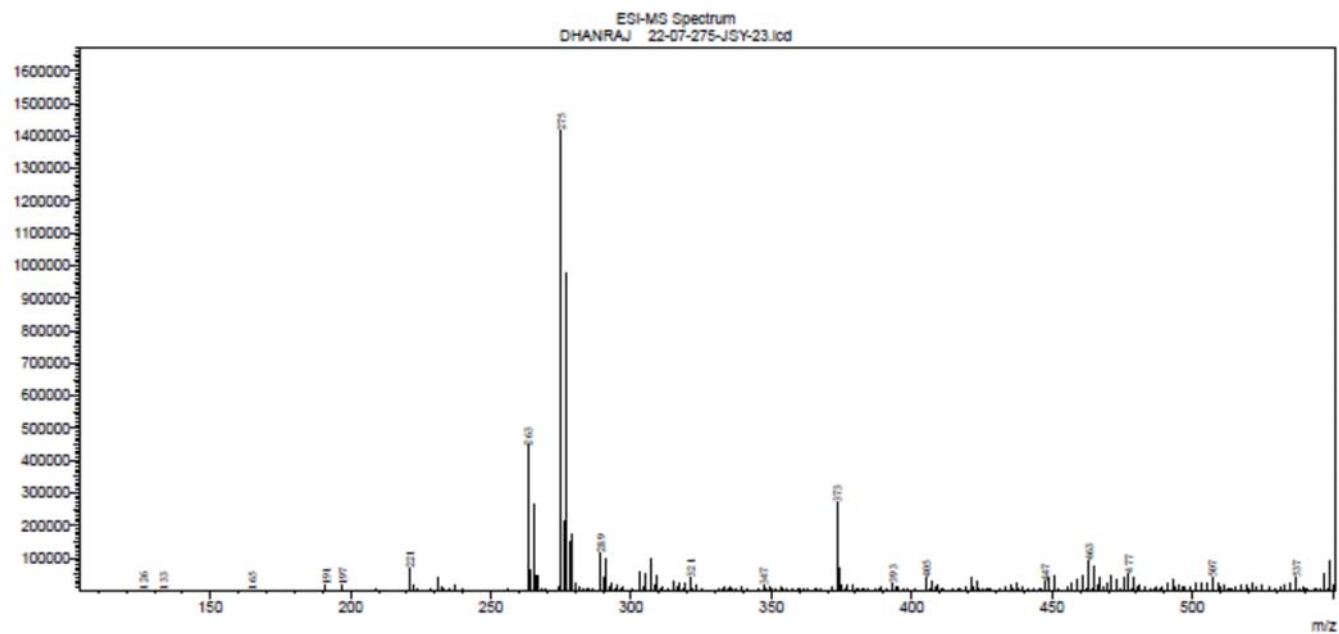
ESI-MS Spectrum of Compound 3k
