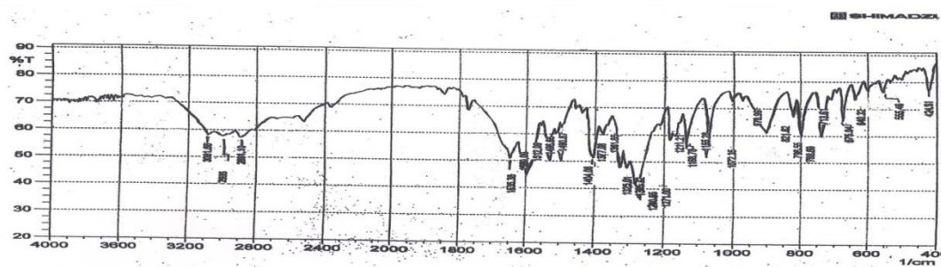
Fig(2)-FT-IR Spectra of compound (7)
