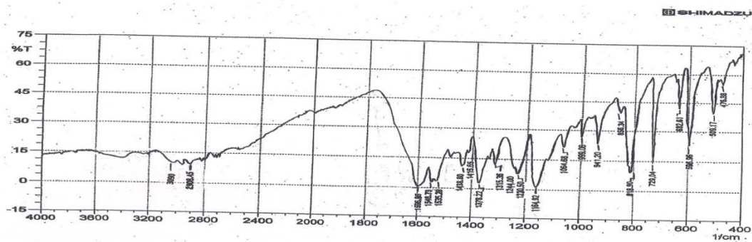
Fig(1)-FT-IR Spectra of compound (6)
