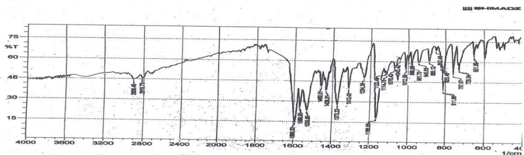
Fig(3)-FT-IR Spectra of compound (8)
